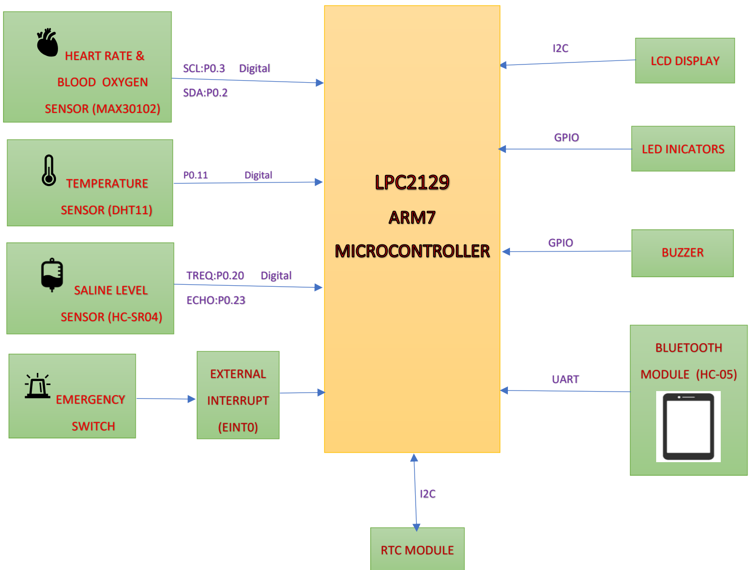
Fig. 3.1 – Block Diagram
